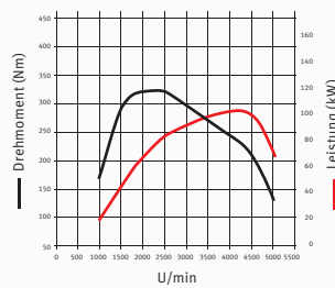
2.0 TDI CR, 103 kW (140 PS)
