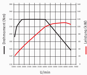
1.4 TSI, 110 kW (150 PS)
